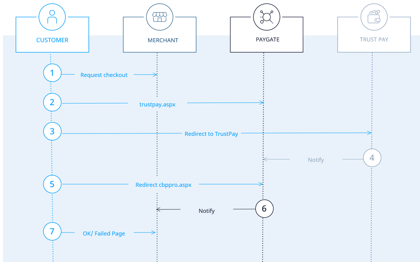
TrustPay process flow
